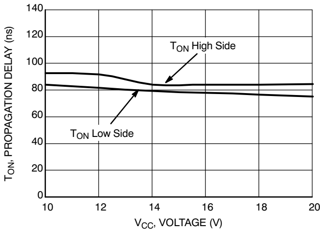
Figure 8. Turn ON Propagation Delay vs. Supply Voltage ( V_{CC} = V_{BOOT} )
